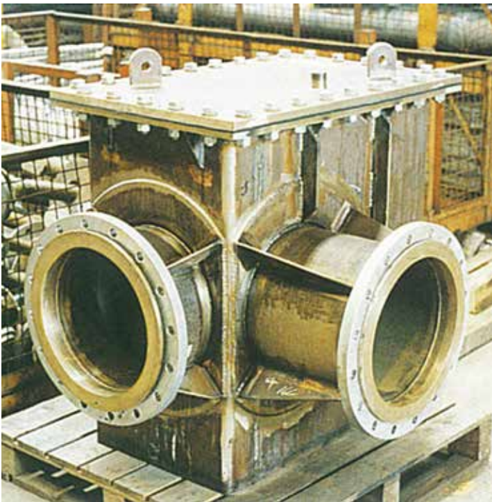
90-10 copper-nickel welded fabrication with flange connections
