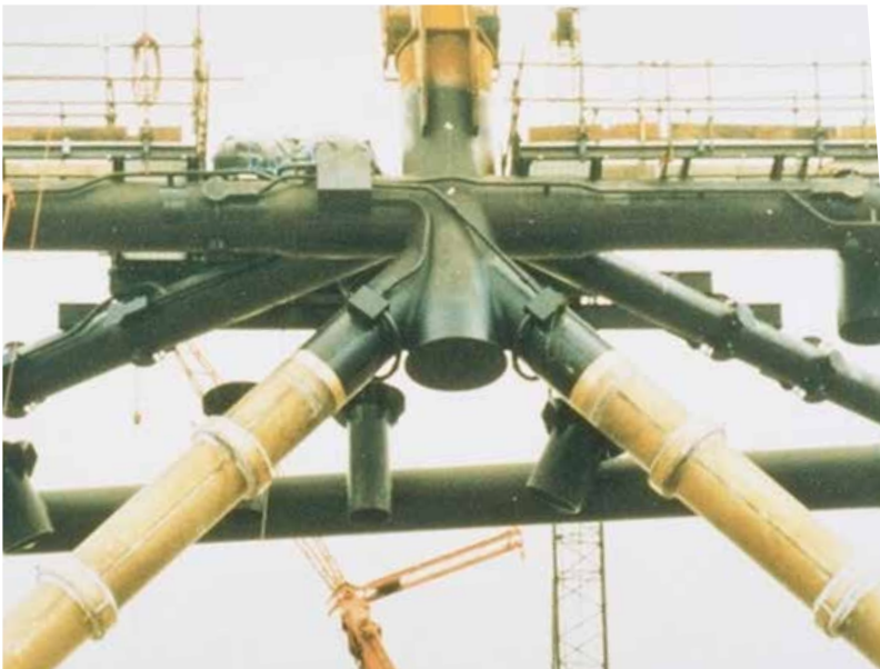
Structural members sheathed in 90-10 copper-nickel during construction of the Phase 1 Morecambe gas field platforms (Courtesy Centrica Energy Upstream, East Irish Sea)
